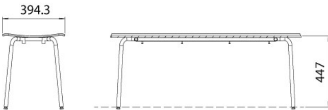
Four Seating Bench 120, Steel frame
