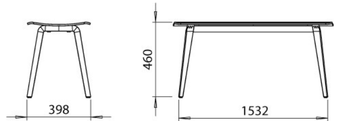
Four Seating Bench 160, Wooden frame
