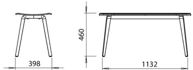
Four Seating Bench 120, Wooden frame
