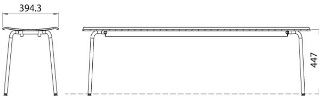
Four Seating Bench 160, Steel frame
