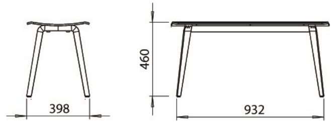
Four Seating Bench 100, Wooden frame
