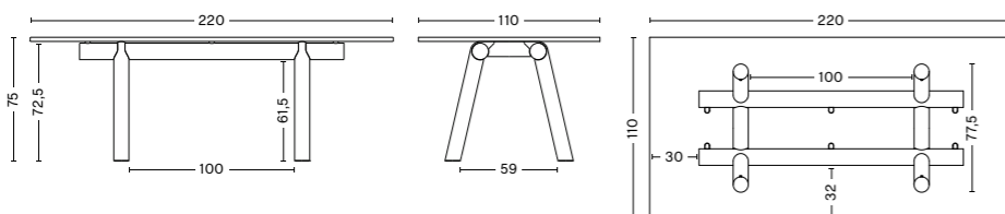
BOA TABLE Width 220 cm Depth 110 cm Height 75 cm
