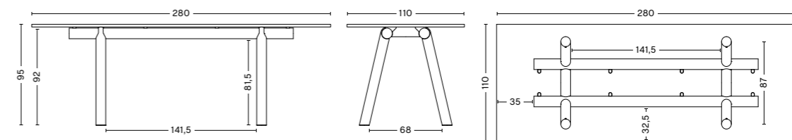
BOA TABLE Width 280 cm Depth 110 cm Height 95 cm
