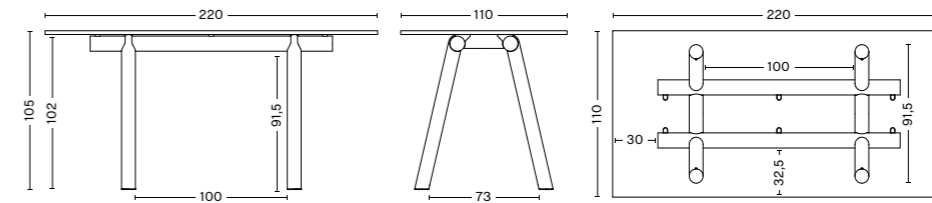
BOA TABLE Width 220 cm Depth 110 cm Height 105 cm
