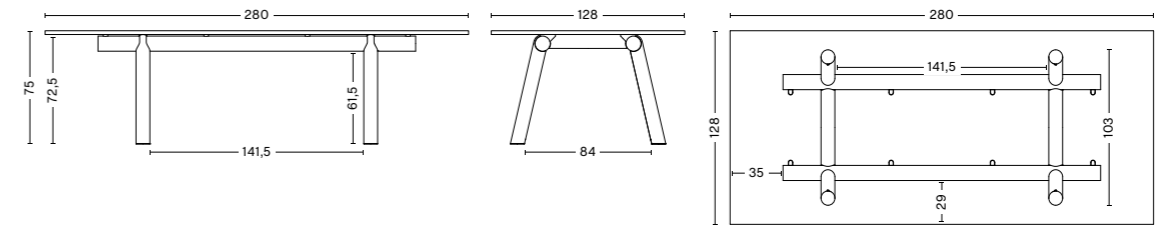
BOA TABLE Width 280 cm Depth 128 cm Height 75 cm
