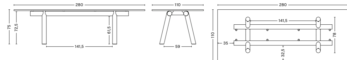
BOA TABLE Width 280 cm Depth 110 cm Height 75 cm
