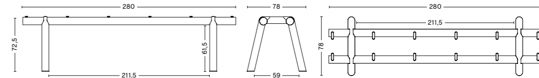
BOA TABLE FRAME Width 280 cm Depth 78 cm Height 72,5 cm
